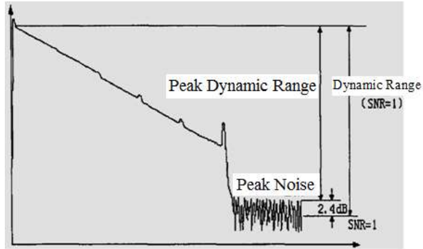
Figure 2-3 Dynamic Range Diagram
