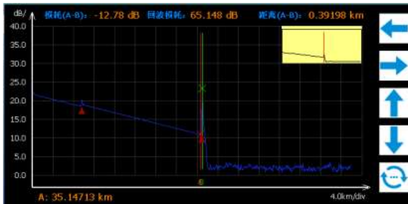
Fig.3-10 Return loss measurement
