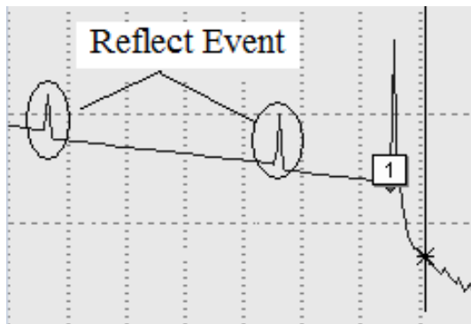
Figure 2-1 Reflection Events Diagram
