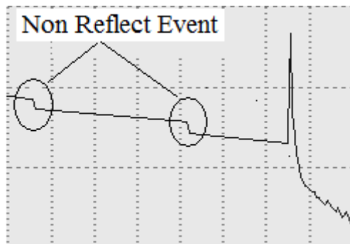
Figure 2-2 Non Reflection Events Diagram
