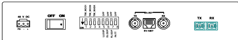
FE1 Fiber Modem/DC Rear Panel Schematic
