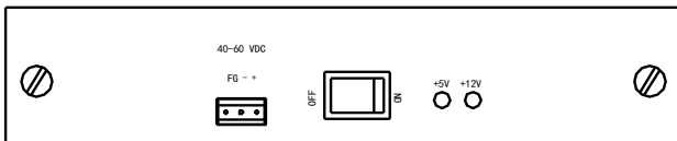
RACK DC Redundancy Power Supply Panel
